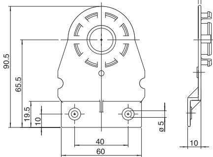
Mounting bracket 6401
