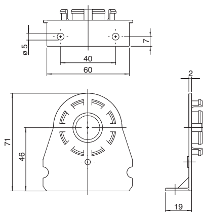
Mounting bracket 6482
