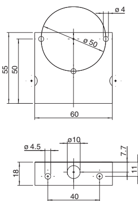
Mounting bracket 6401
