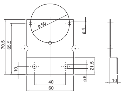
Mounting bracket 6402
